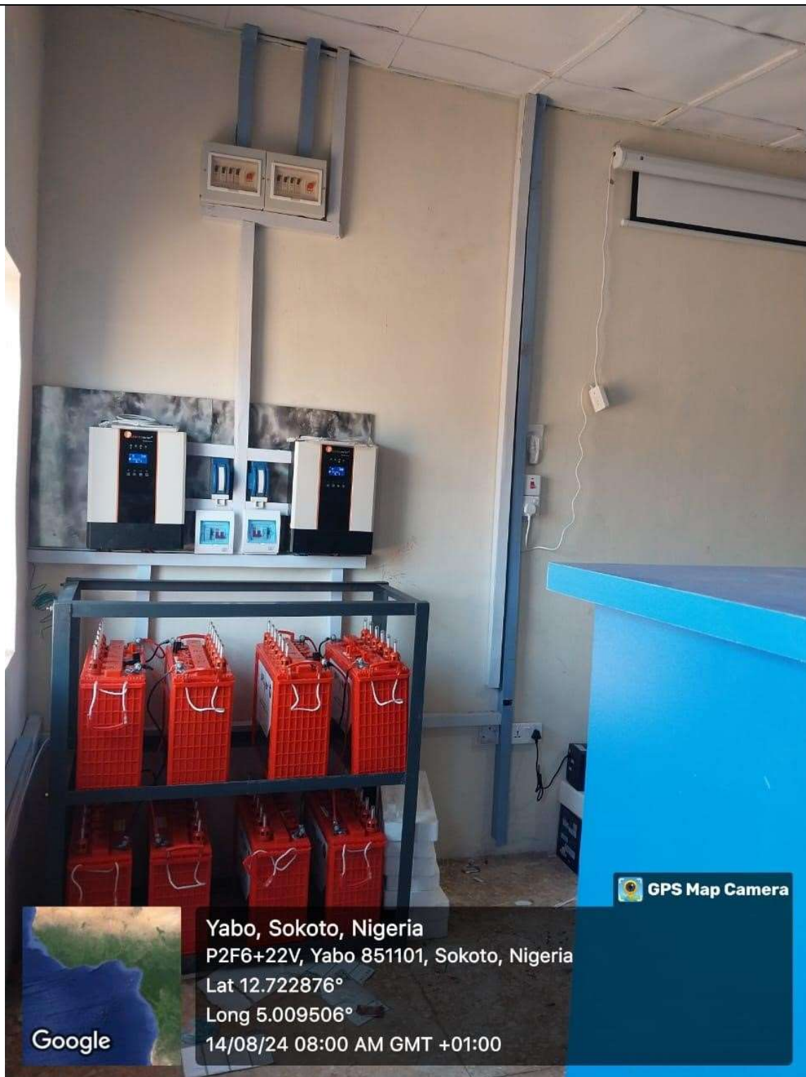
INSTALLED INVERTERS AND BATTERIES
