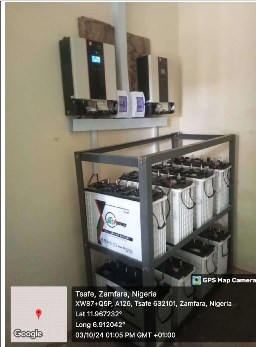
INSTALLED BATTERIES & INVERTERS AND FIRE EXTINGUISHER
